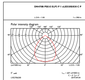
OFPC1_DN470BPSE-EELP3P1xLED20S830CP
