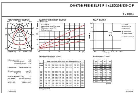
IFGU1_DN470BPSE-EELP3P1xLED20S830CP
